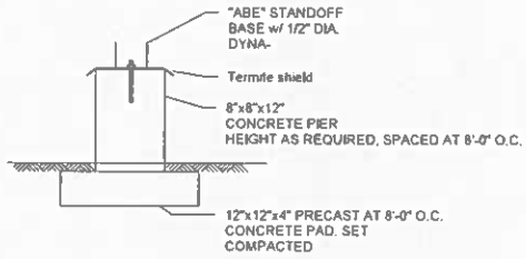
② Typical Footing at Elevated Floor1 1" = 1'-0"
