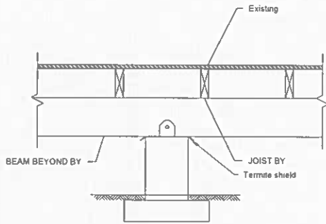
① Footing at Elevated Floor 1" = 1'-0"
