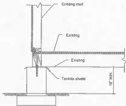
③ Footing at Elevated Floor2 1" = 1'-0"
