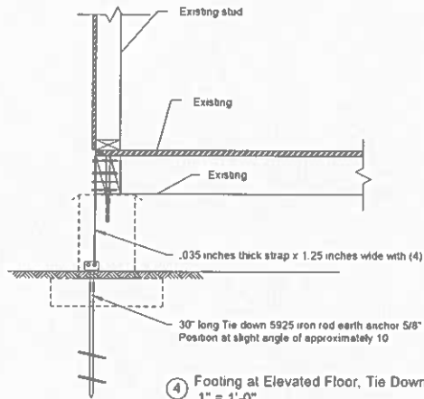
④ Footing at Elevated Floor, Tie Down 1" = 1'-0"
